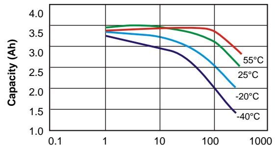
Capacity versus Current and Temperature
